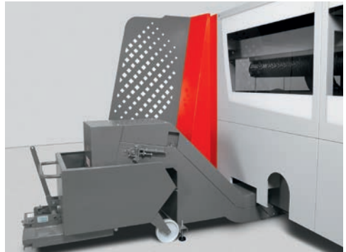
Teileauswurf über Querförderer in Container. Discharge of parts into the container by the cross conveyor.
