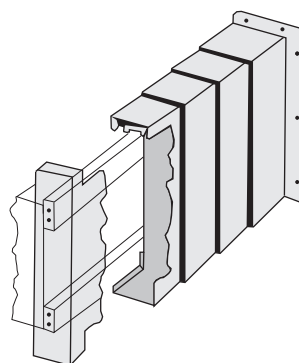
Querbalkenabdeckung Transverse beam cover
