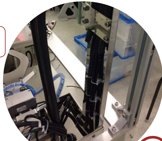
Vertical running FLATVEYOR®
