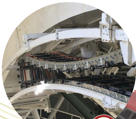
Shutter systems
