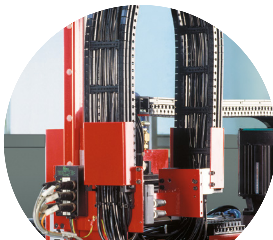
Vertical running QUANTUM cable carrier
